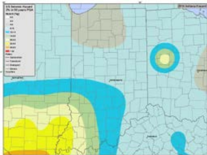
Figure 23 Indiana Seismic Zone Map
